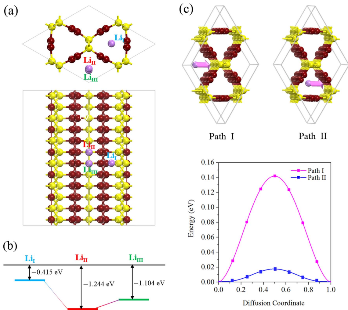
Fig. 6. (a) Top and side views of the possible Li absorption sites. (b) Binding energies of the three configurations in (a). (c) Considered migration paths of Li diffusion and the corresponding diffusion energy barrier profiles.
