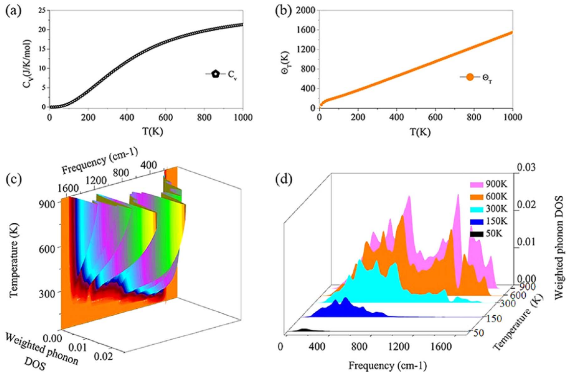
Fig. 4. (a) Heat capacity, and (b) Debye temperature of the Hex- C_{18} with respect to temperature; (c) 3D plot of the weighted phonon DOS as a function of frequency and temperature; (d) cross sections of the weighted phonon DOS at 50, 150, 300, 600, and 900 K.
