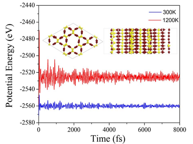
Fig. 3. Total potential energy fluctuation during AIMD simulation at 300 K and 1200 K. The inset shows the atomic configurations (2×2×4 supercell) at the end of AIMD simulations at 1200 K.
