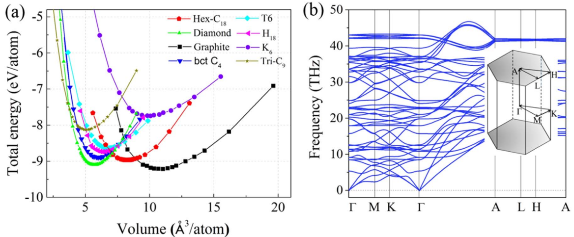
Fig. 2. (a) Volume dependence of total energy per atom for Hex-C 18 , diamond, graphite, bct C 4 , T6, H 18 , K 6 , and Tri-C 9 carbons. (b) Phonon band structure of Hex-C 18 . The inset shows the first Brillouin zone and the high symmetry k point path.
