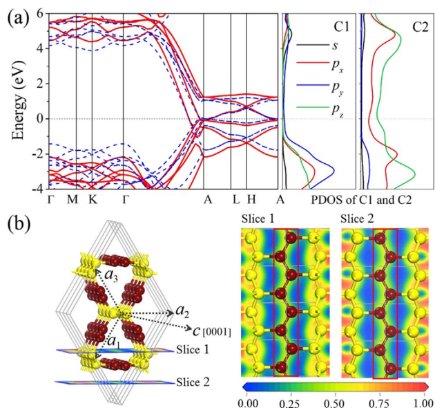
Fig. 5. (a) Electronic band structures calculated using the DFT-GGA/PBE (blue dashed lines) and the HSE06 hybrid functional (red solid lines), and projected DOS for C1 and C2 atom at DFT-GGA/PBE level of Hex-C 18 . (b) Two ELF slices parallel to the (10\bar{1}0) crystal surface of Hex-C 18 .
