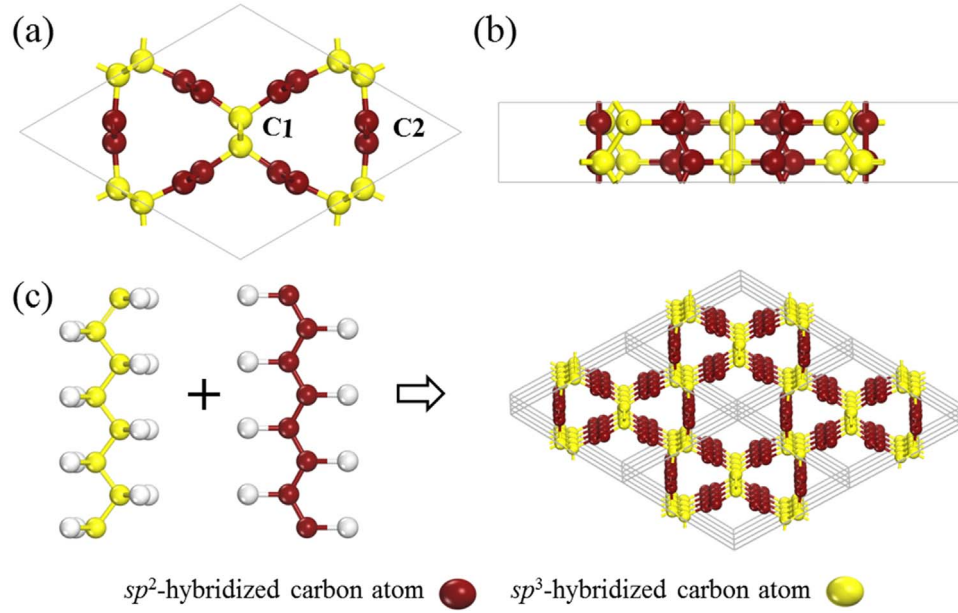
Fig. 1. (a) Top view and (b) side view of the optimized structure of Hex-C 18 . (c) A schematic illustration of a possible synthesis strategy for Hex-C 18 by using C-H chains via dehydrogenation and assembly.
