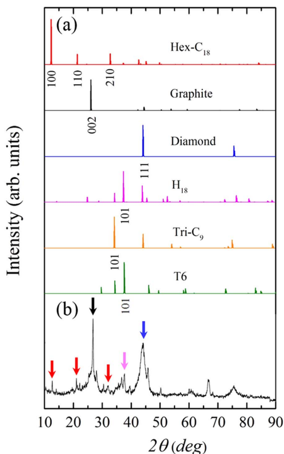
Fig. 7. Simulated XRD patterns for (a) Hex-C 18 , graphite, diamond, H 18 , Tri-C 9 , and T6 carbons. (b) Experimental XRD pattern for the detonation soot of TNT (sample Alaska B [58]). Red, pink, black, and blue arrows indicate the peaks that match the simulated characteristic peaks of Hex-C 18 , H 18 , graphite, and diamond, respectively. The X-ray wavelength we adopted for simulation is 1.54059 Å.
